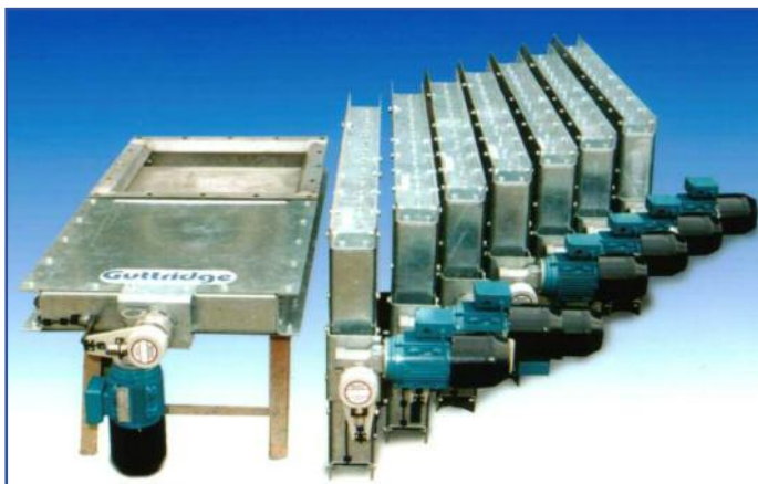
Motorised slide valves
